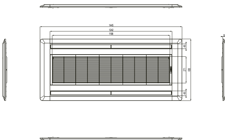
TE01 panel
