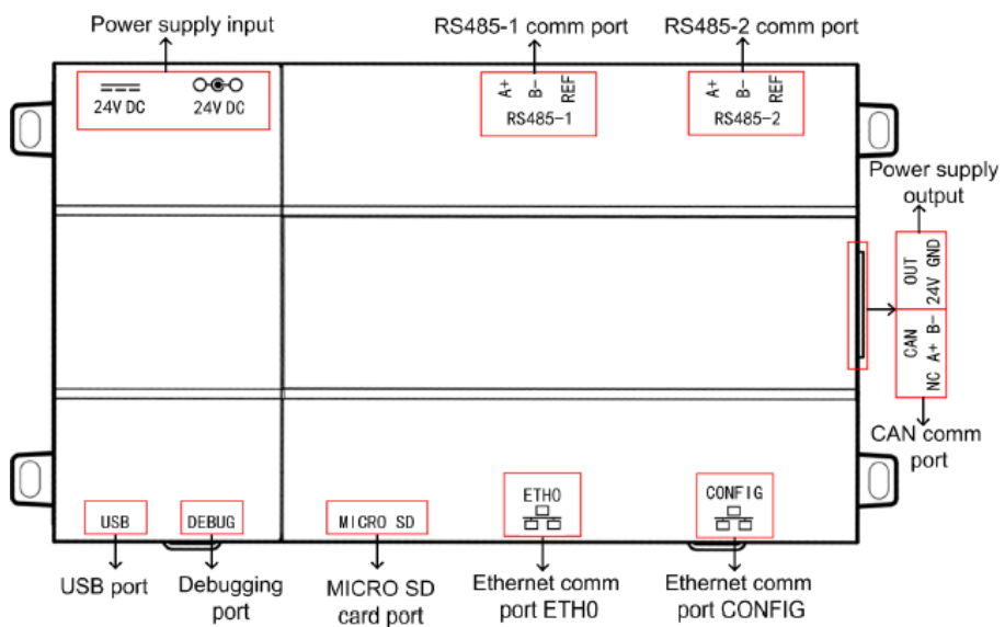
Diagram of Interface Function
