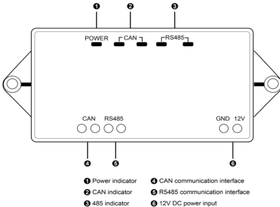
Diagram of Modbus Gateway
