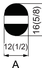
Mounting hole drawing
