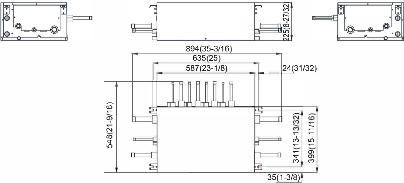
Unit outline dimension: mm (in.)
